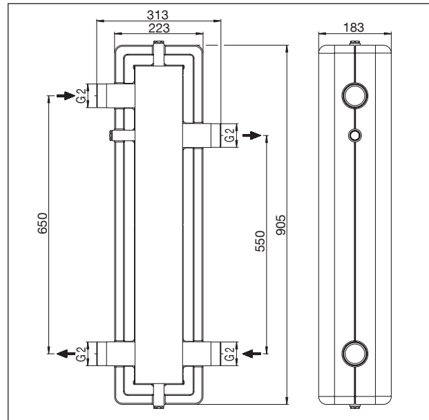
Dimensions hydronic header DN 32
